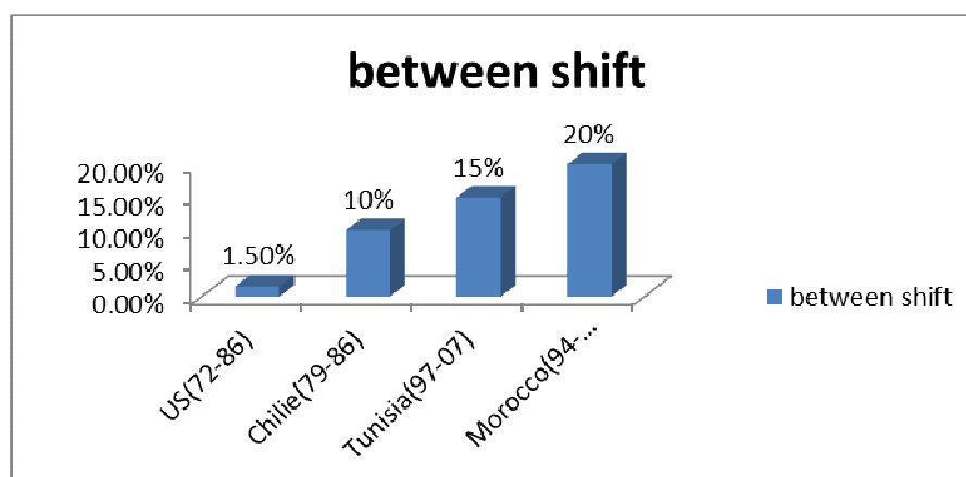
Figure 7: fraction of between shift comparison (manufacturing)
